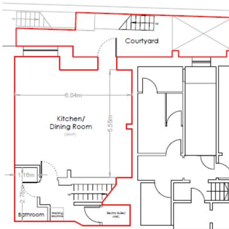
Lower Ground Floor scale 1:100
