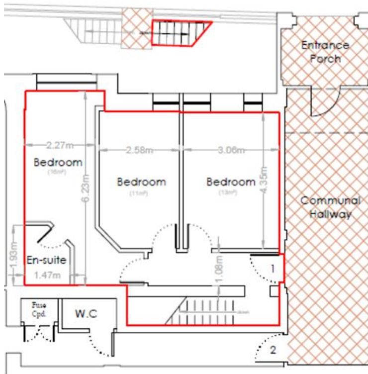
Ground Floor scale 1:100
